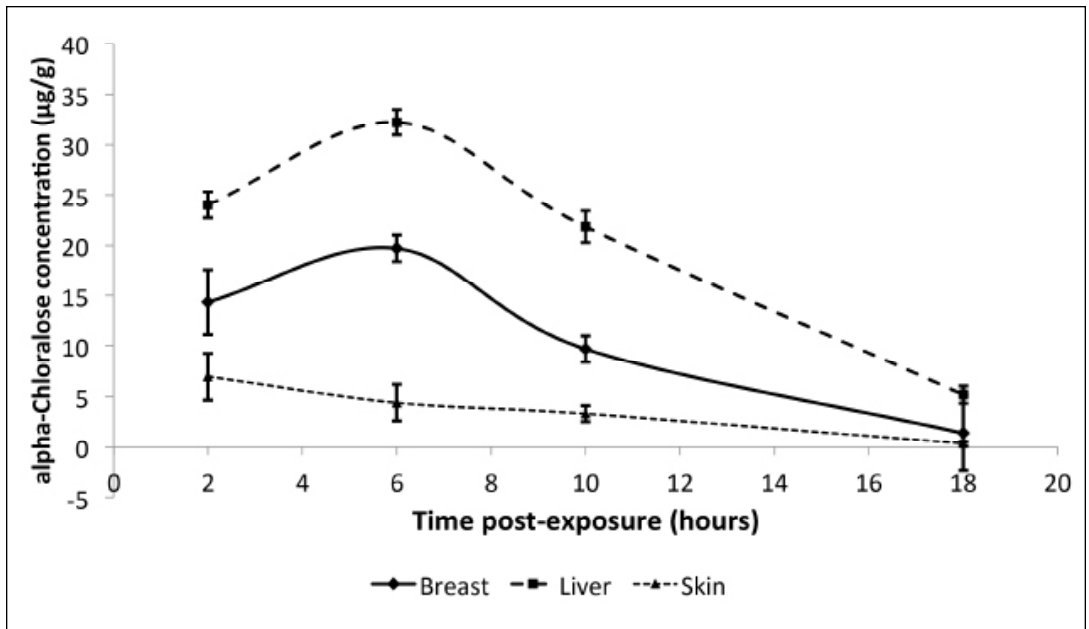
Figure 1. Elimination of radio-labeled alpha-chloralose (AC) and metabolites from mallard ducks ( Anas platyrhynchos ) following a single oral dose ( n = 3 /time point). Values plotted are means \pm 1 standard deviation.
